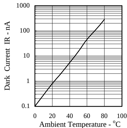
FIG.4 DARK CURRENT VS AMBIENT TEMPERATURE
