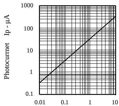
FIG.6 PHOTOCURRENT VS. IRRADIANCE = 950 nm
