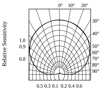
FIG.7 SENSITIVITY DIAGRAM
