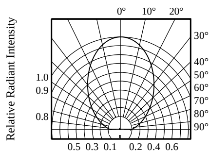
FIG.5 RADIATION DIAGRAM
