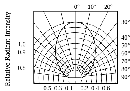
FIG.5 RADIATION DIAGRAM
