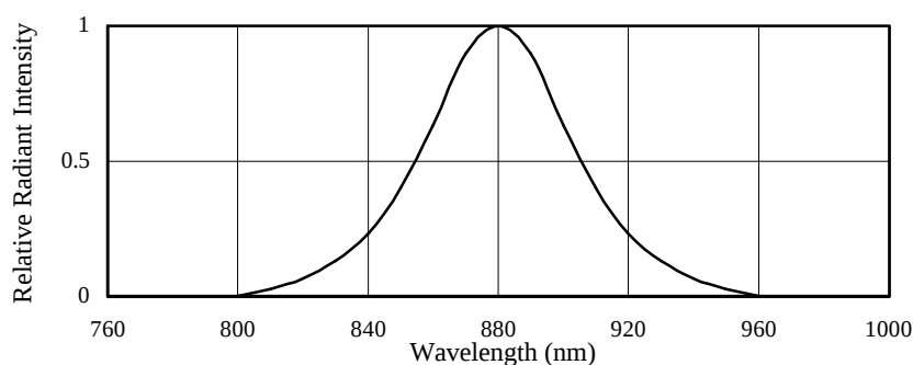
FIG.1 SPECTRAL DISTRIBUTION
