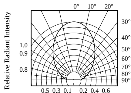
FIG.5 RADIATION DIAGRAM
