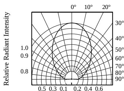
FIG.5 RADIATION DIAGRAM
