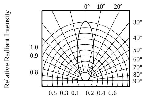
FIG.5 RADIATION DIAGRAM
