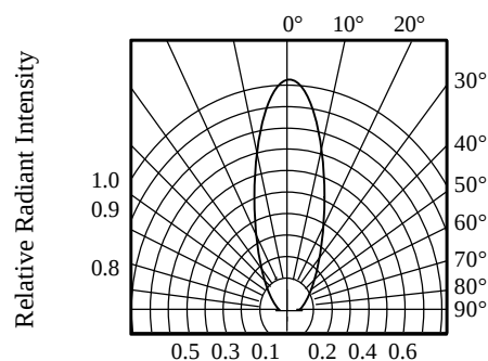
FIG.5 RADIATION DIAGRAM
