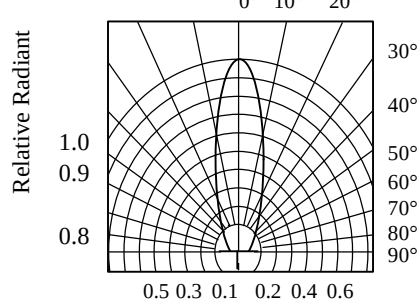
FIG.6 RADIATION DIAGRAM
