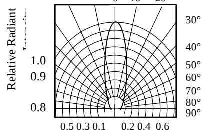
FIG.6 RADIATION DIAGRAM
