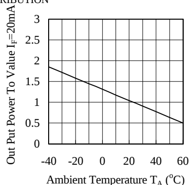
FIG.3 RELATIVE RADIANT INTENSITY VS. AMBIENT TEMPERATURE
