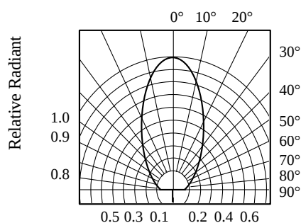
FIG.6 RADIATION DIAGRAM
