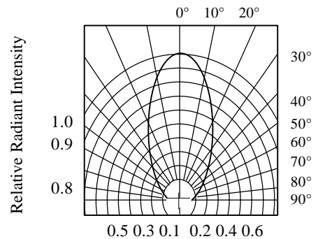
FIG.5 RADIATION DIAGRAM
