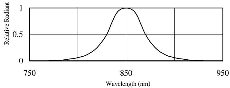
FIG.1 SPECTRAL DISTRIBUTION
