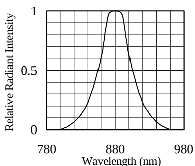
FIG.1 SPECTRAL DISTRIBUTION
