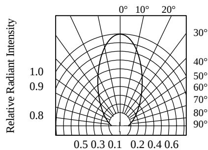
FIG.6 RADIATION DIAGRAM
