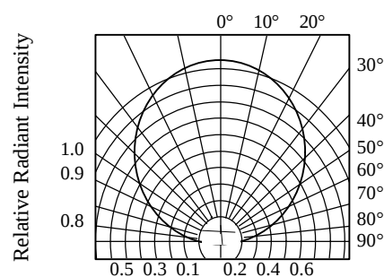
FIG.6 RADIATION DIAGRAM
