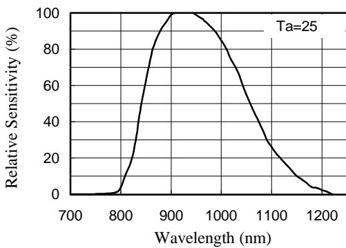
Fig.9 Spectral Sensitivity (Detecting side)
