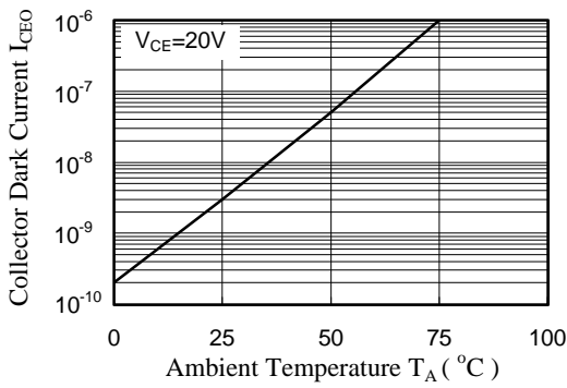
Fig.7 Collector Dark Current vs. Ambient Temperature
