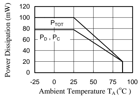
Fig.2 Power Dissipation vs. Ambient Temperature
