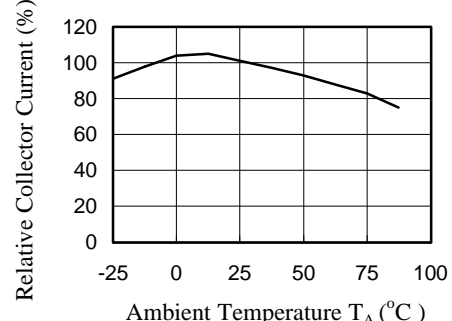
Fig.6 Relative Collector Current vs. T A
