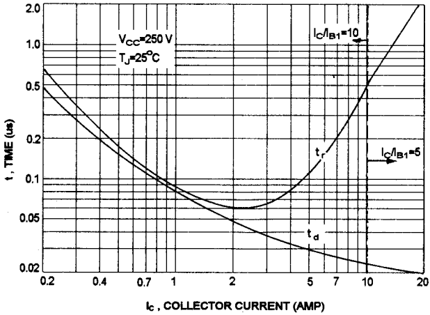
TURN-ON TIME
