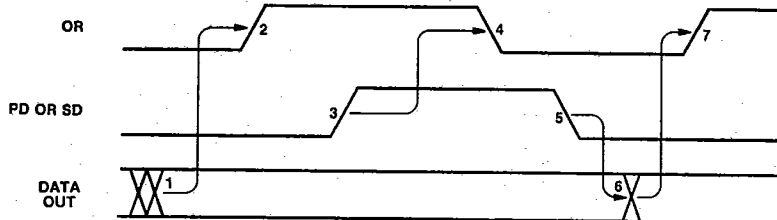
MJ2812HS OUTPUT TIMING
