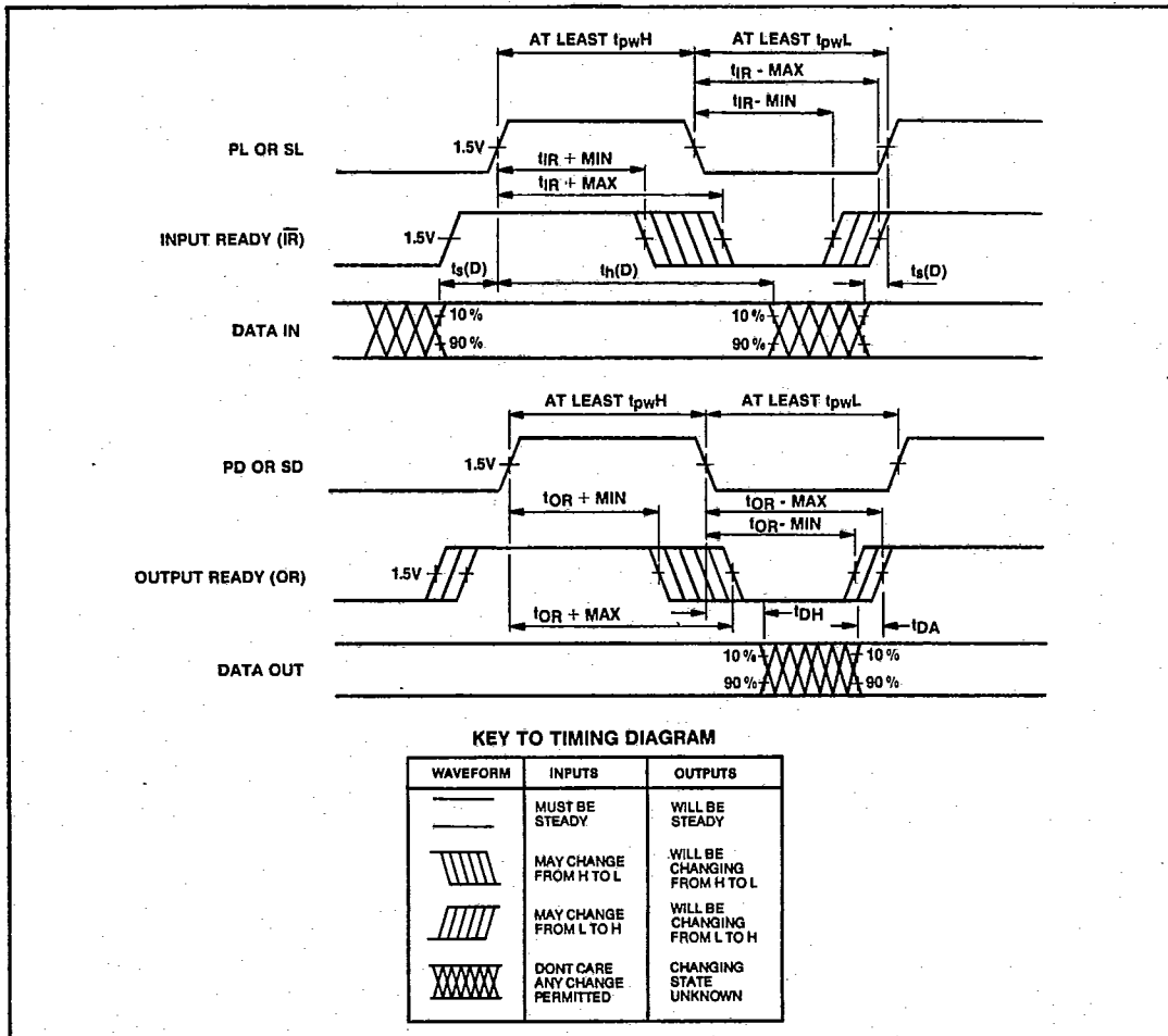
Fig.5 Timing diagram
