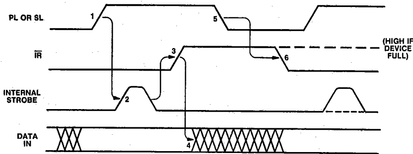
MJ2812HS INPUT TIMING
