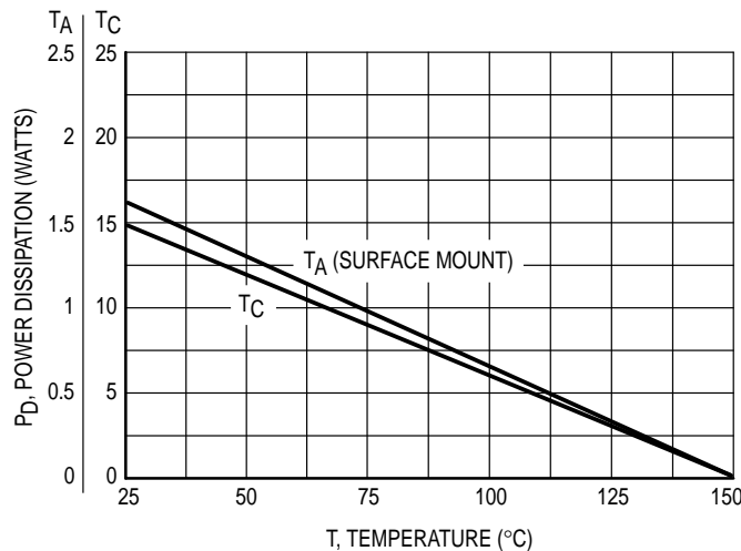
Figure 7. Power Derating
