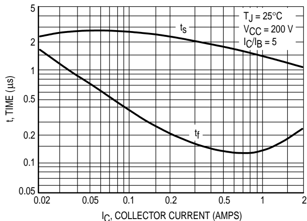
Figure 4. Turn-Off Time
