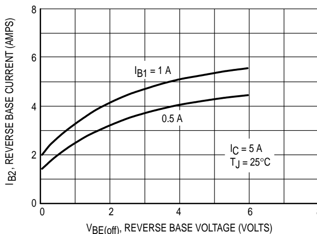
Figure 13. Peak Reverse Base Current
