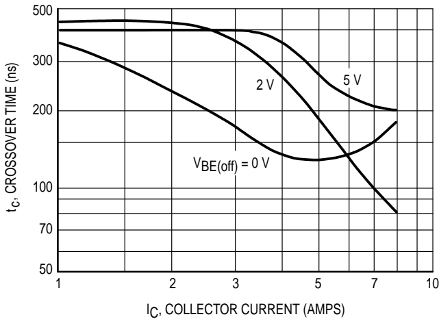
Figure 10. Crossover Time
