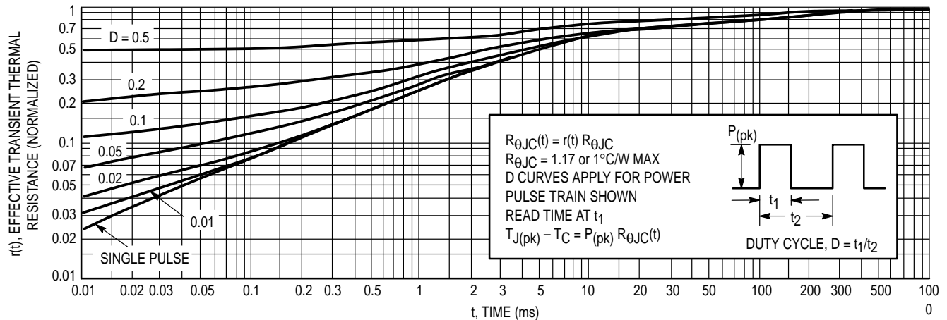
Figure 18. Thermal Response
