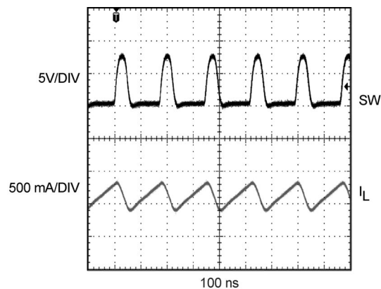
Typical Switching Waveform ( V_{IN} = 3.6V , 4LEDs, 1\mu H )
