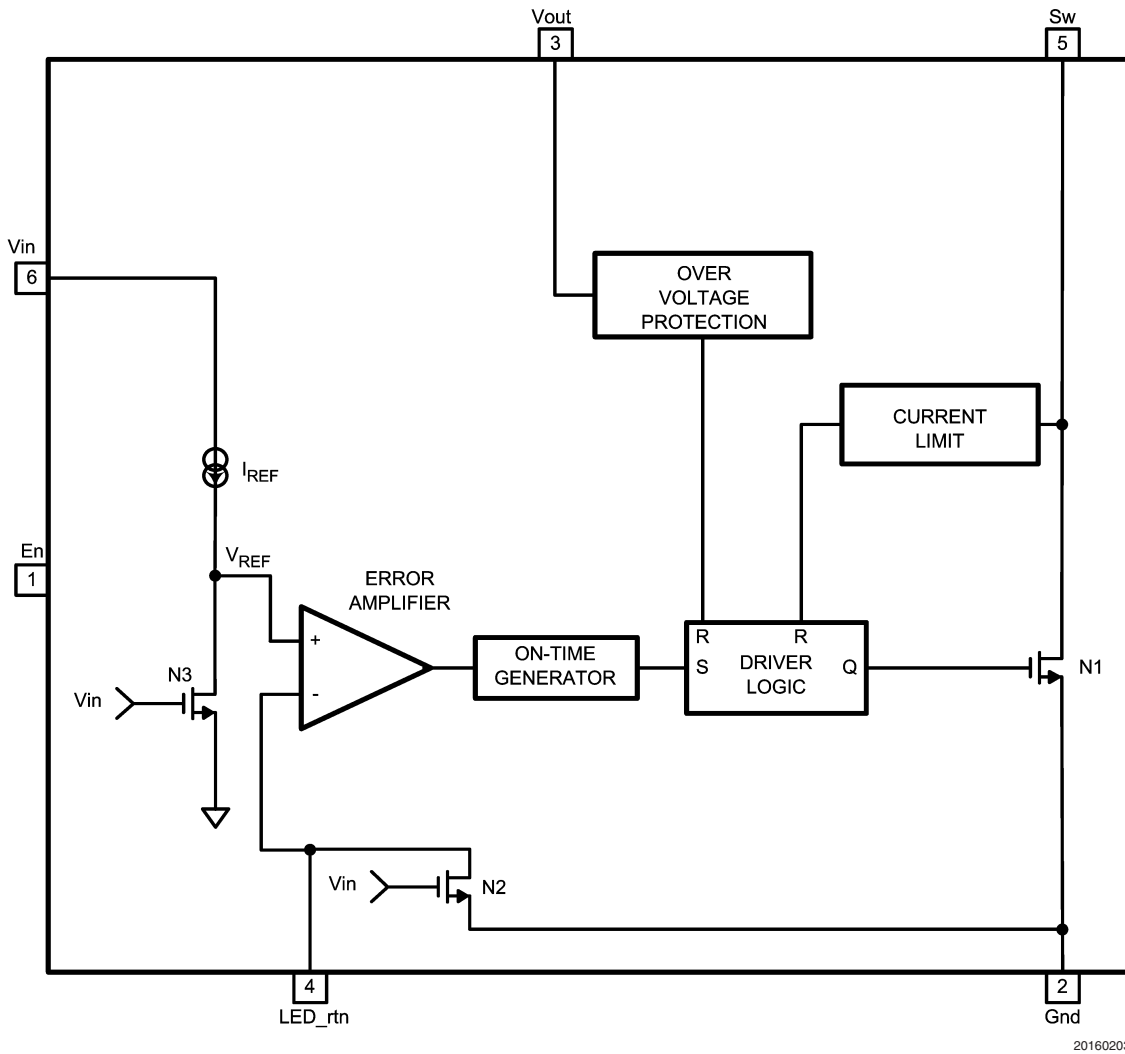
FIGURE 2. Block Diagram
