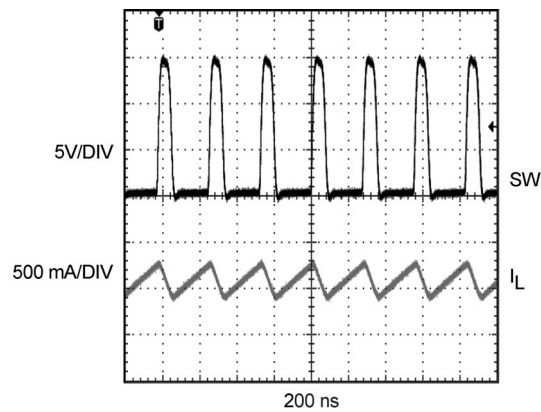
Typical Switching Waveform ( V_{IN} = 3.6V , 4LEDs, 2.2\mu H )
