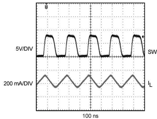
Typical Switching Waveform ( V_{IN} = 3.6V , 2LEDs, 2.2\mu H )
