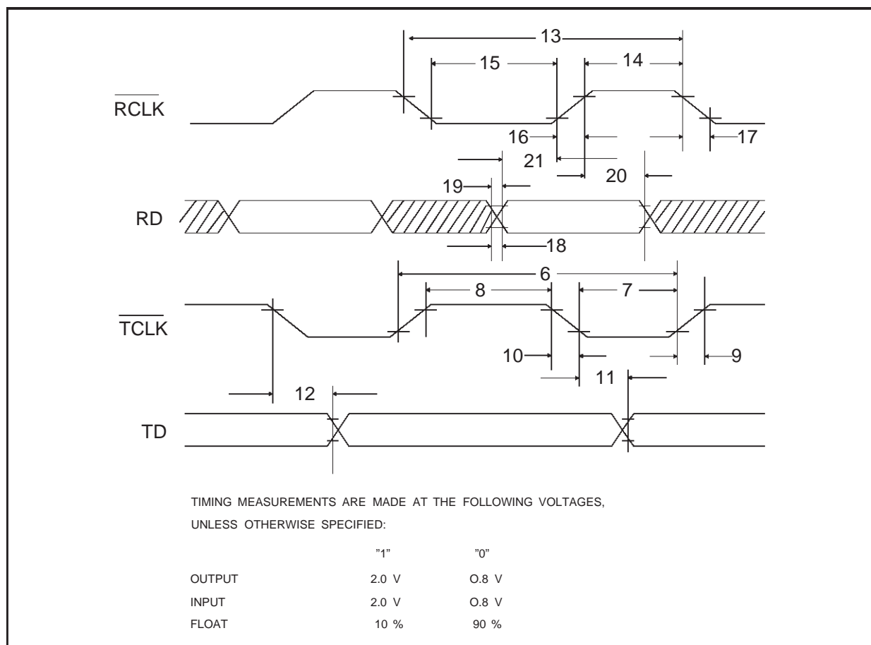
Figure 10: MK50H28 Serial Link Timing Diagram
