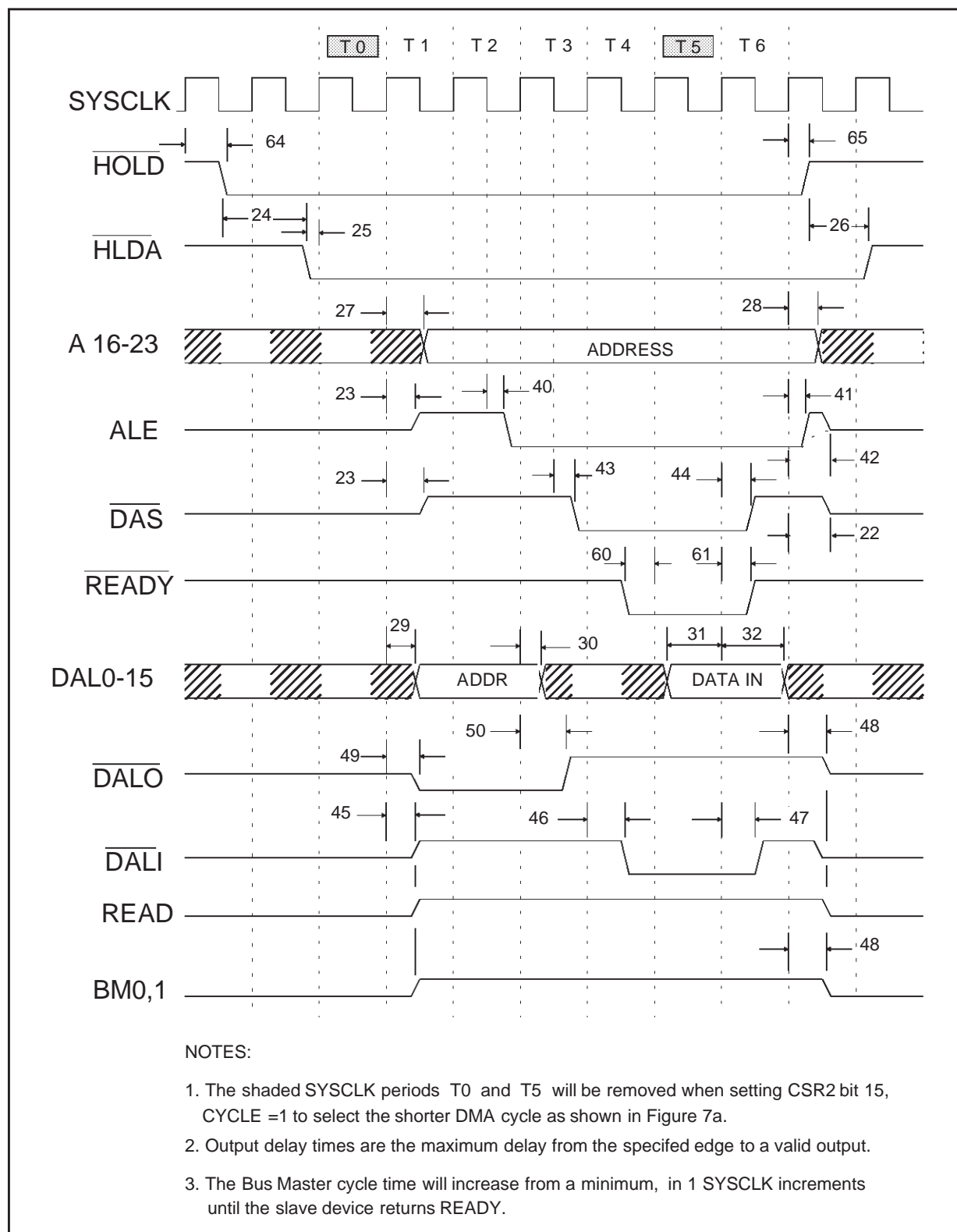
Figure 11: MK50H28 BUS Master Timing (Read) (for CYCLE = 0, CSR2&lt;15&gt;)
