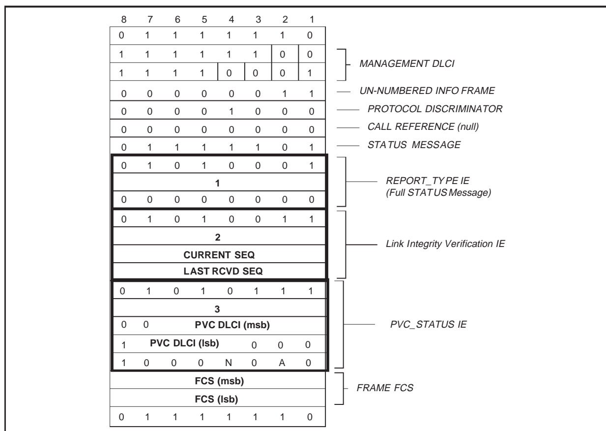
Figure 5: Sample Annex A STATUS Frame (Full)
