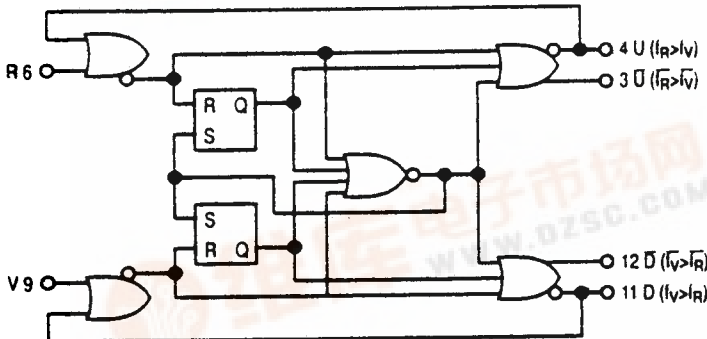
LOGIC DIAGRAM
