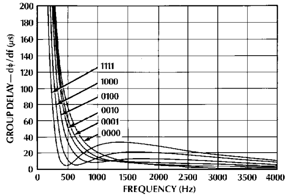
Figure 3. Typical Slope Filter Response — NL/L = 1
