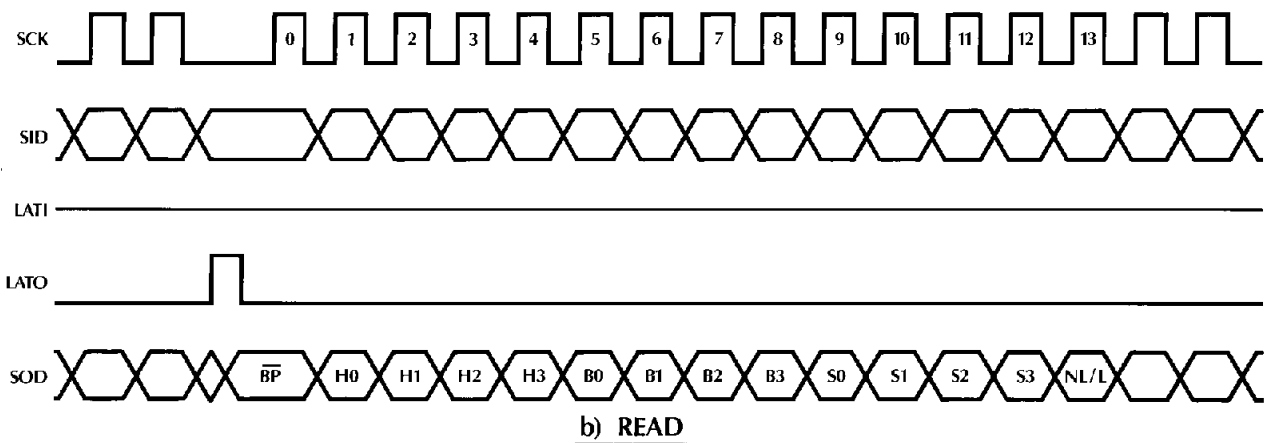
Figure 6. Serial Timing
