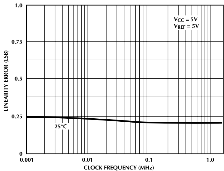
Figure 2. Linearity Error vs f CLK
