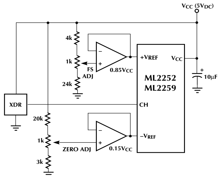
Figure 9. Operating with Ratiometric Transducers 15% of V_{CC} - V_{XDR} - 85\% of V_{CC}
