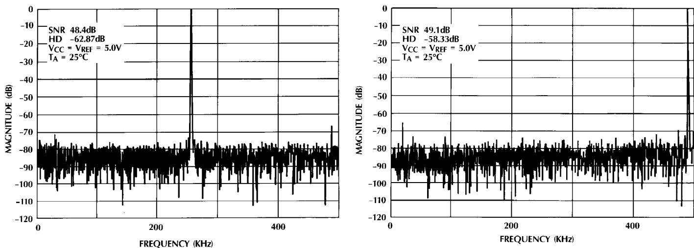
a) Ouput Spectrum with f_{IN} = 257\text{kHz} , f_S = 1\text{MHz} b) Output Spectrum with f_{IN} = 491\text{kHz} , f_S = 1\text{MHz}
