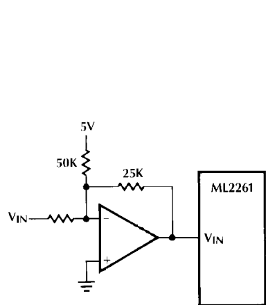
Figure 15. \pm 2.5V Analog Input Range
