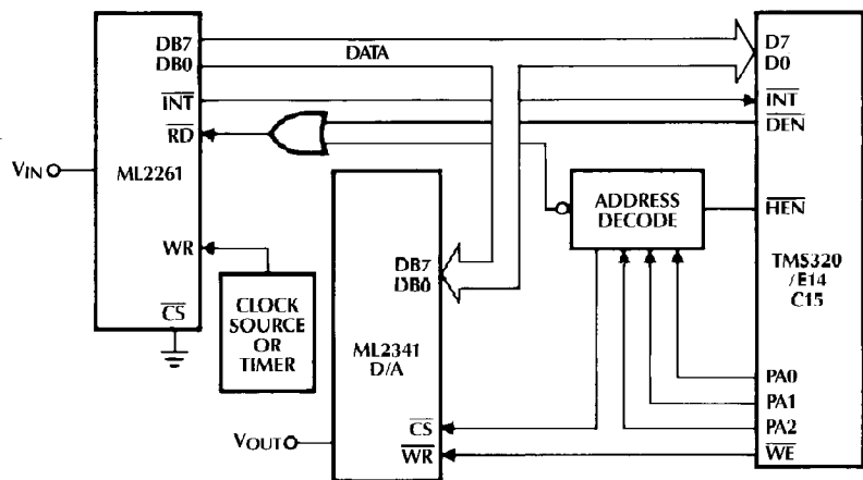
Figure 17. TMS320 Interface with D/A Output
