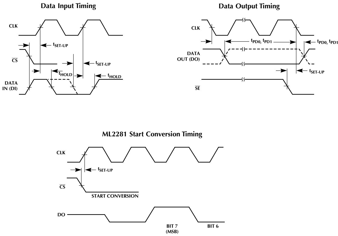
Figure 2. Timing Diagrams
