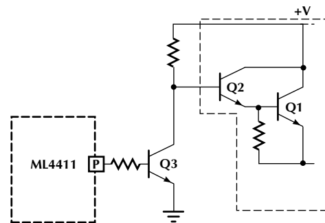
Figure 20. High Voltage Translation with NPN Darlington
