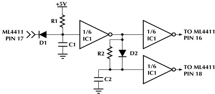
Figure 11. Analog Start-up Circuit
