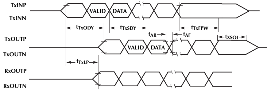
Figure 3. Transmit Timing
