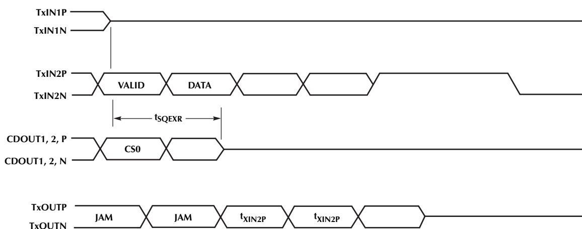
Figure 6. Collision Timing
