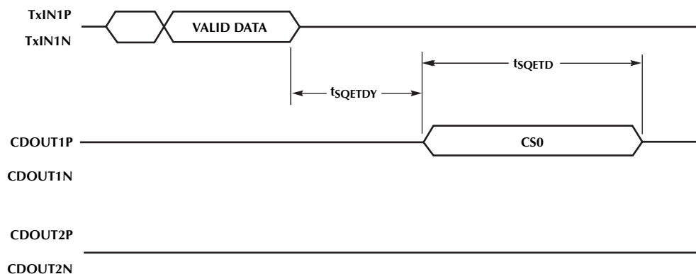
Figure 7. SQE Timing
