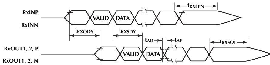
Figure 4. Receive Timing
