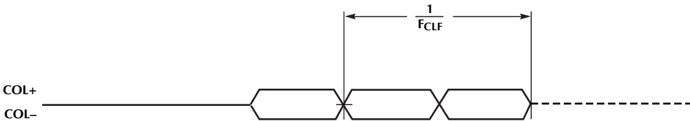
Figure 10. Collision Timing
