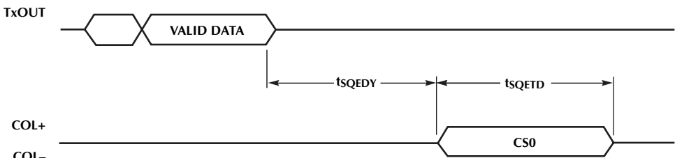
Figure 11. SQE Timing
