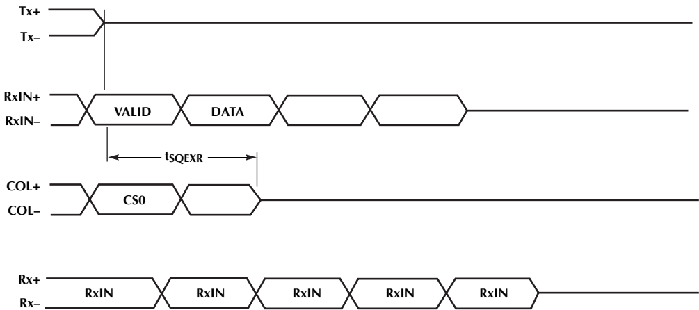
Figure 9. Collision Timing
