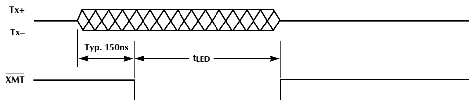
Figure 13. LED Timing
