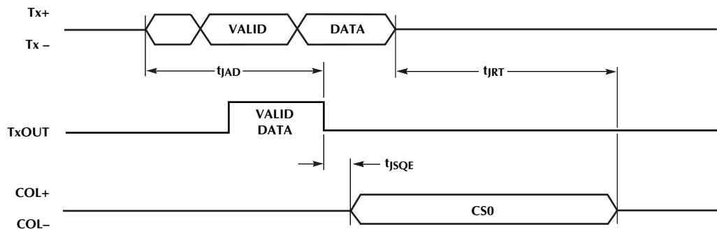
Figure 12. Jabber Timing
