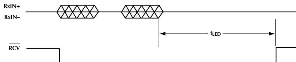
Figure 14. LED Timing
