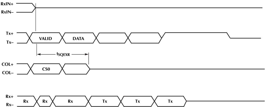
Figure 8. Collision Timing
