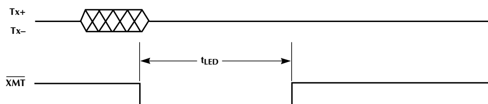
Figure 15. LED Timing
