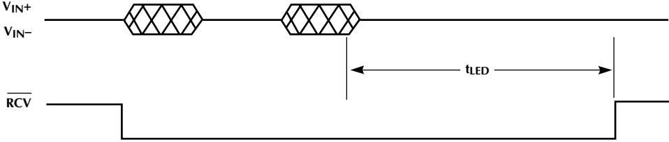
Figure 16. LED Timing
