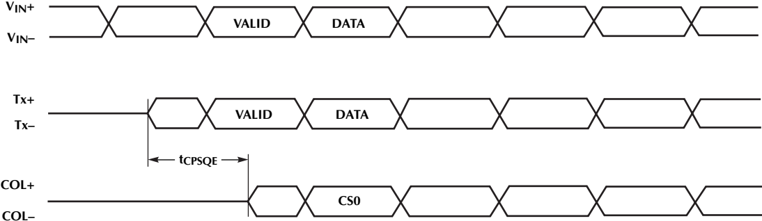
Figure 9. Collision Timing
