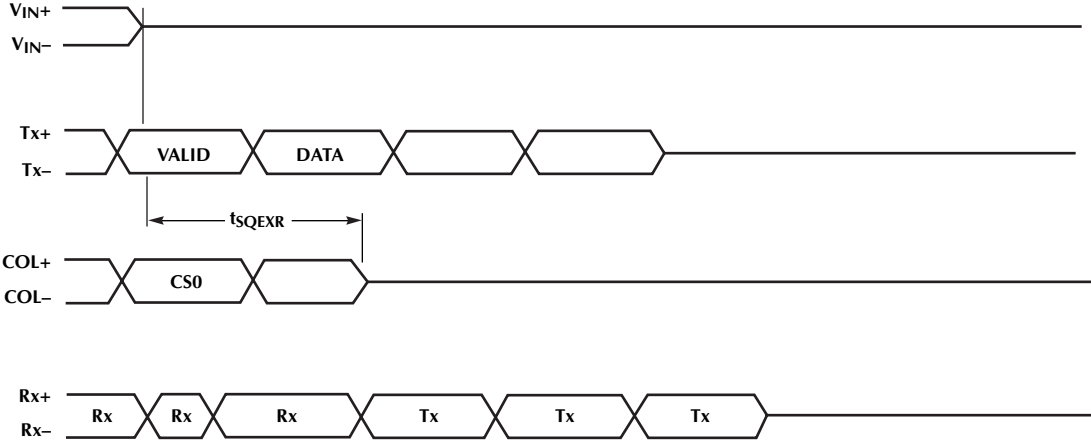
Figure 10. Collision Timing
