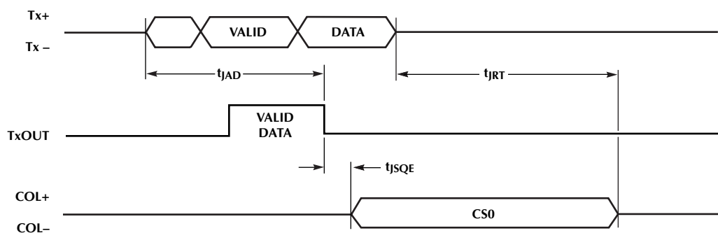
Figure 14. Jabber Timing
