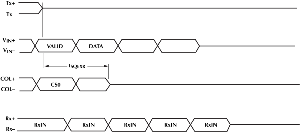
Figure 11. Collision Timing
