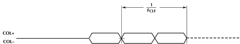
Figure 12. Collision Timing
