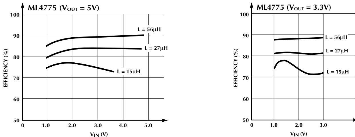
Figure 5. Typical Efficiency as a Function of V IN .
