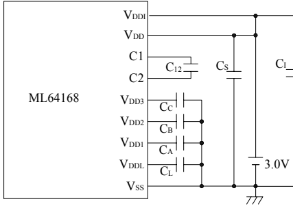
ML64168 3.0V Version.(The LCD bias is regulated.)
