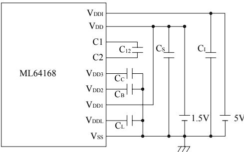
ML64168 1.5V Version
