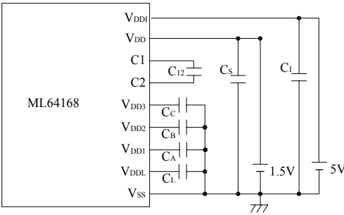
ML64168 1.5V Version.(The LCD bias is regulated.)
