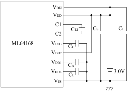
ML64168 3.0V Version
