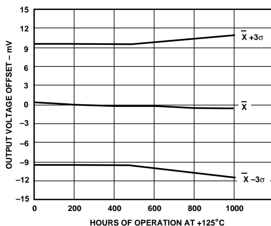
Figure 41. Output Voltage Offset ( Z_{Oj} ) Distribution Accelerated by Burn-in
