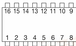
SOP-16A
