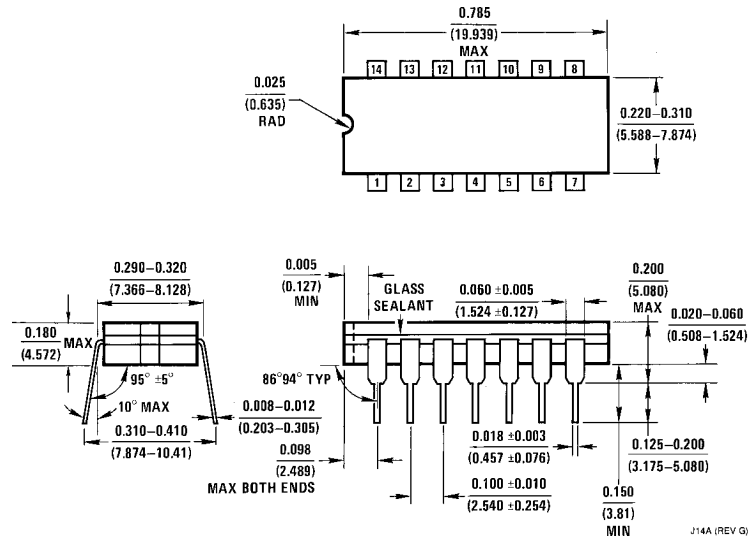
Ceramic Dual-In-Line Package (J) Order Number MM54C00J, MM54C02J, MM54C04J, MM54C10J, MM54C20J, MM74C00J, MM74C02J, MM74C04J, MM74C10J or MM74C20J NS Package Number J14A
