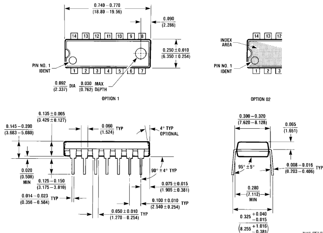
Ceramic Dual-In-Line Package (J) Order Number MM54C74N or MM74C74N NS Package Number N14A
