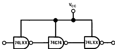
74C Compatibility
