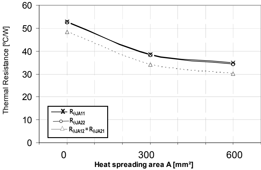
Figure 21. Device on Thermal Test Board R_{\theta JA}
