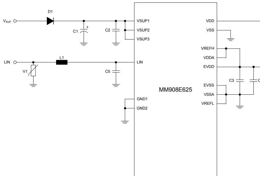
Figure 17. EMC/EMI recommendations
