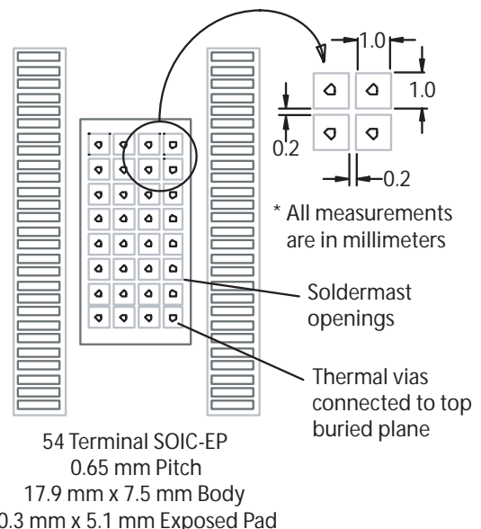
Figure 19. Thermal Land Pattern for Direct Thermal Attachment Per JEDEC JESD51-5 Thermal Test Board
