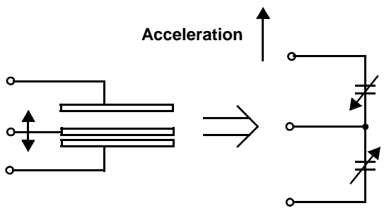
Figure 2. Transducer Physical Model
