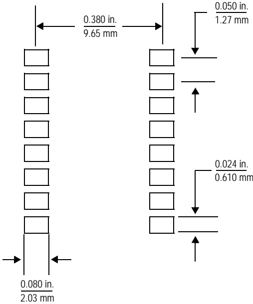
Figure 5. Footprint SOIC-16 (Case 475-01)
