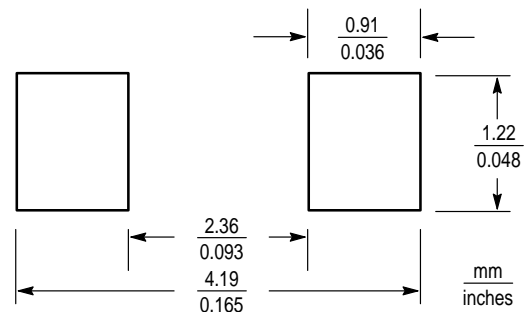
SOD-123
