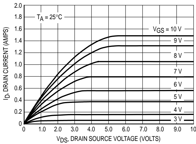
Figure 3. Ohmic Region
