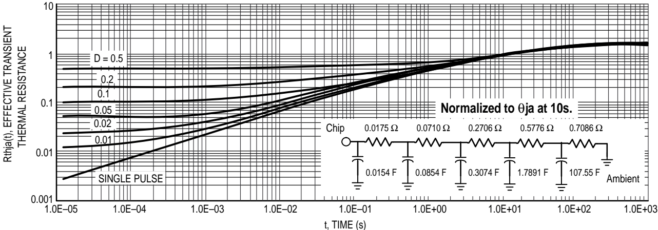
Figure 13. Thermal Response
