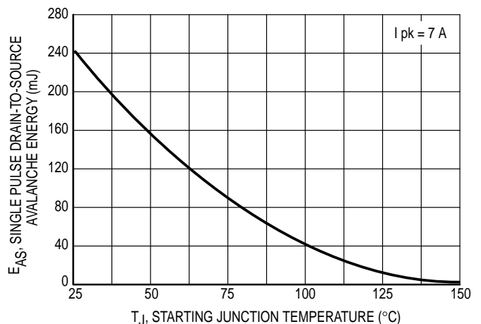
Figure 9. Maximum Avalanche Energy versus Starting Junction Temperature
