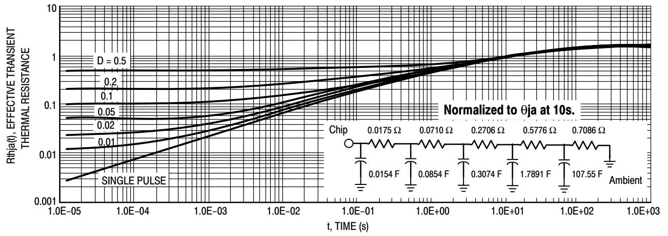
Figure 14. Thermal Response
