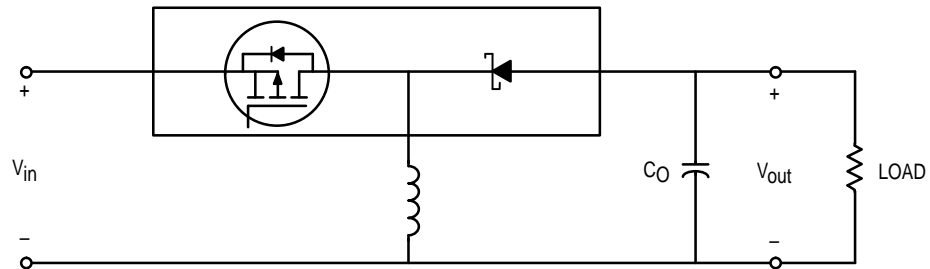
Buck-Boost Regulator
