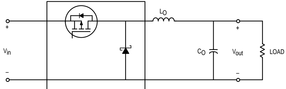
Buck Regulator
