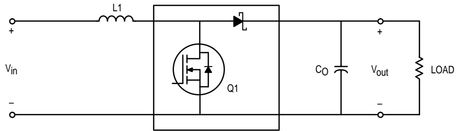
Boost Regulator
