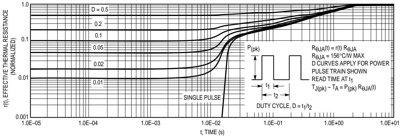
Figure 8. Thermal Response
