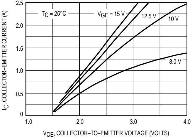
Figure 1. Saturation Characteristics
