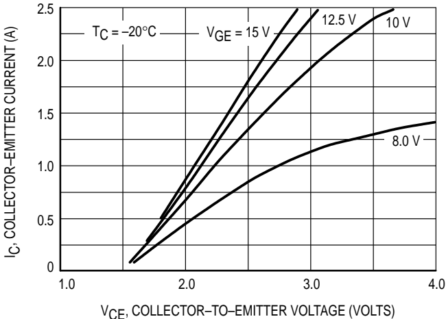
Figure 3. Saturation Characteristics
