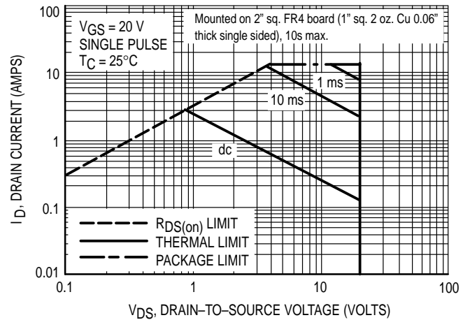
Figure 12. Maximum Rated Forward Biased Safe Operating Area
